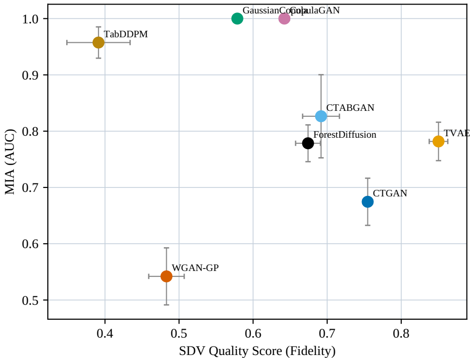
Metro Interstate: SDV Quality Score (Fidelity) vs MIA (AUC)
